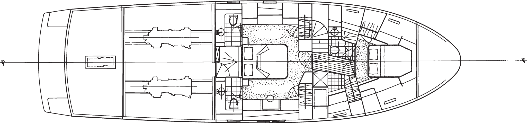
Passage Maker 62 - Lower
